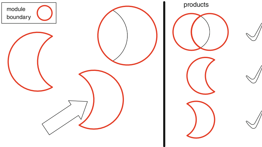
Fig. 9.8 Multiple implementations to make features optional
