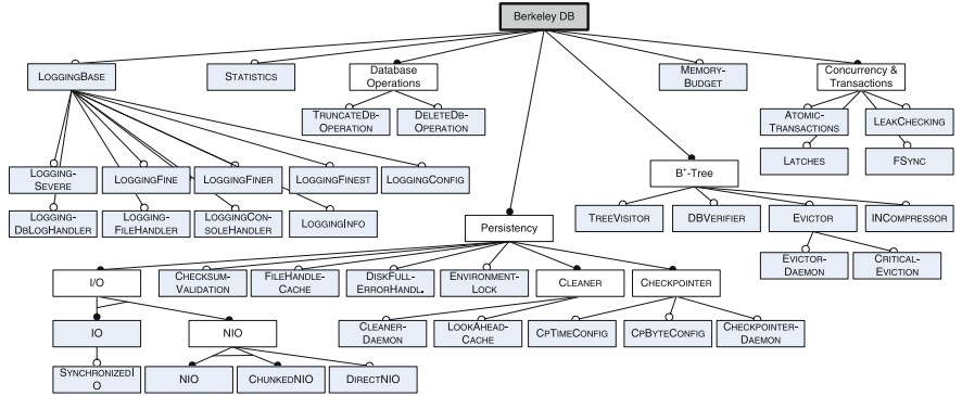
Fig. 8.11 Feature diagram of Berkeley DB after feature extraction
