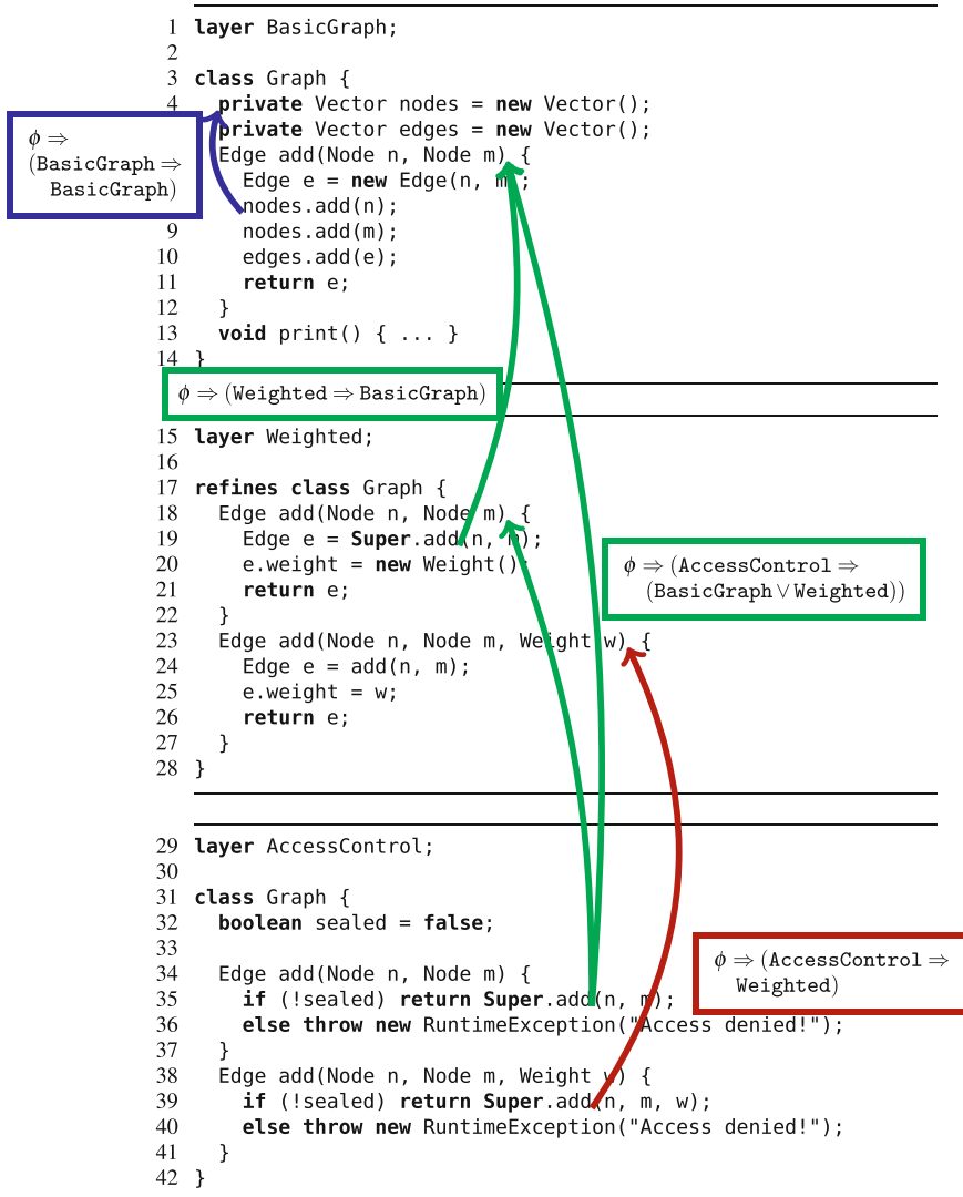
Fig. 10.13 Checking whether references to add are well-typed in all products
