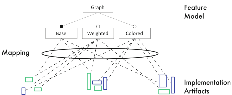
Fig. 7.1 Tool-managed mapping between features and implementation artifacts using tracing links (dashed lines)
