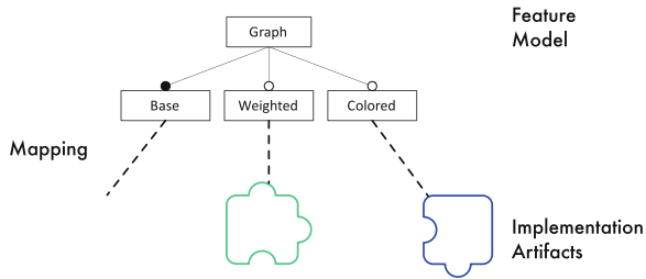
Fig. 6.1 Mapping between features and implementation artifacts in feature-oriented programming
