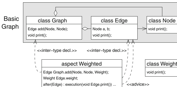
Fig. 6.23 Implementing a collaboration as an aspect
