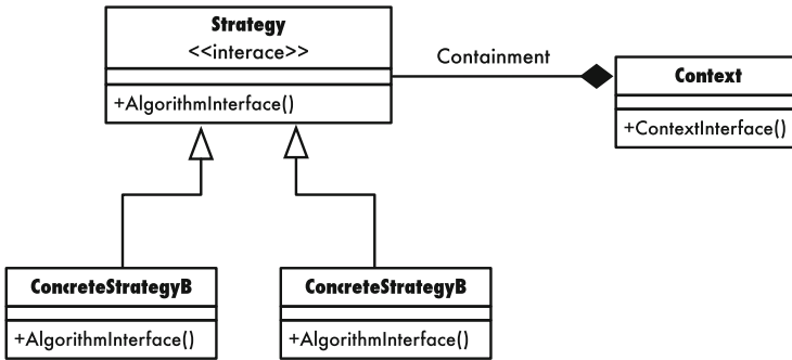
Fig. 4.5 Strategy pattern
