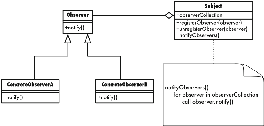
Fig. 4.2 Observer pattern
