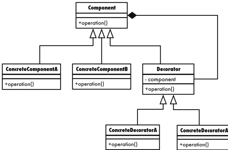
Fig. 4.7 Decorator pattern
