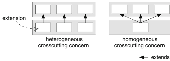
Fig. 6.18 Homogeneous versus heterogeneous crosscutting concerns
