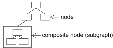
Fig. 6.31 A recursive graph data structure (Apel 2007)
