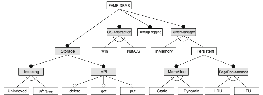
Fig. 9.16 Initial feature model of FAME-DBMS
